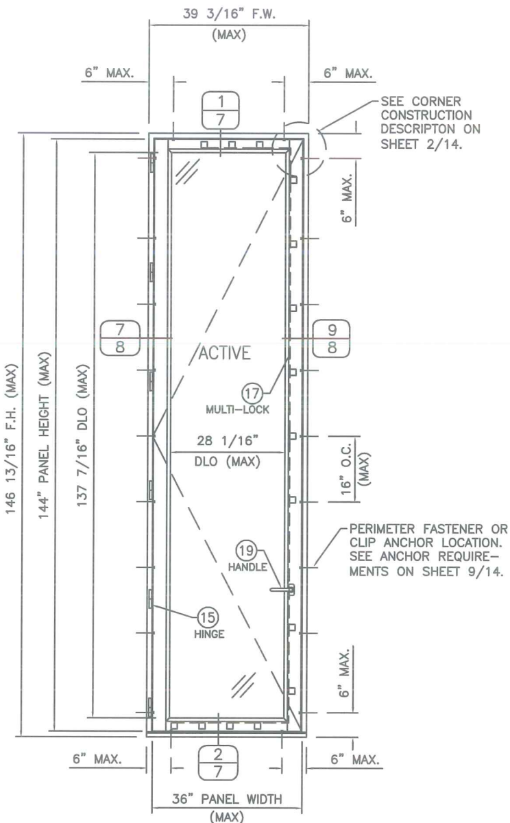
SINGLE RECTANGULAR DOOR (EXTERIOR VIEW)
