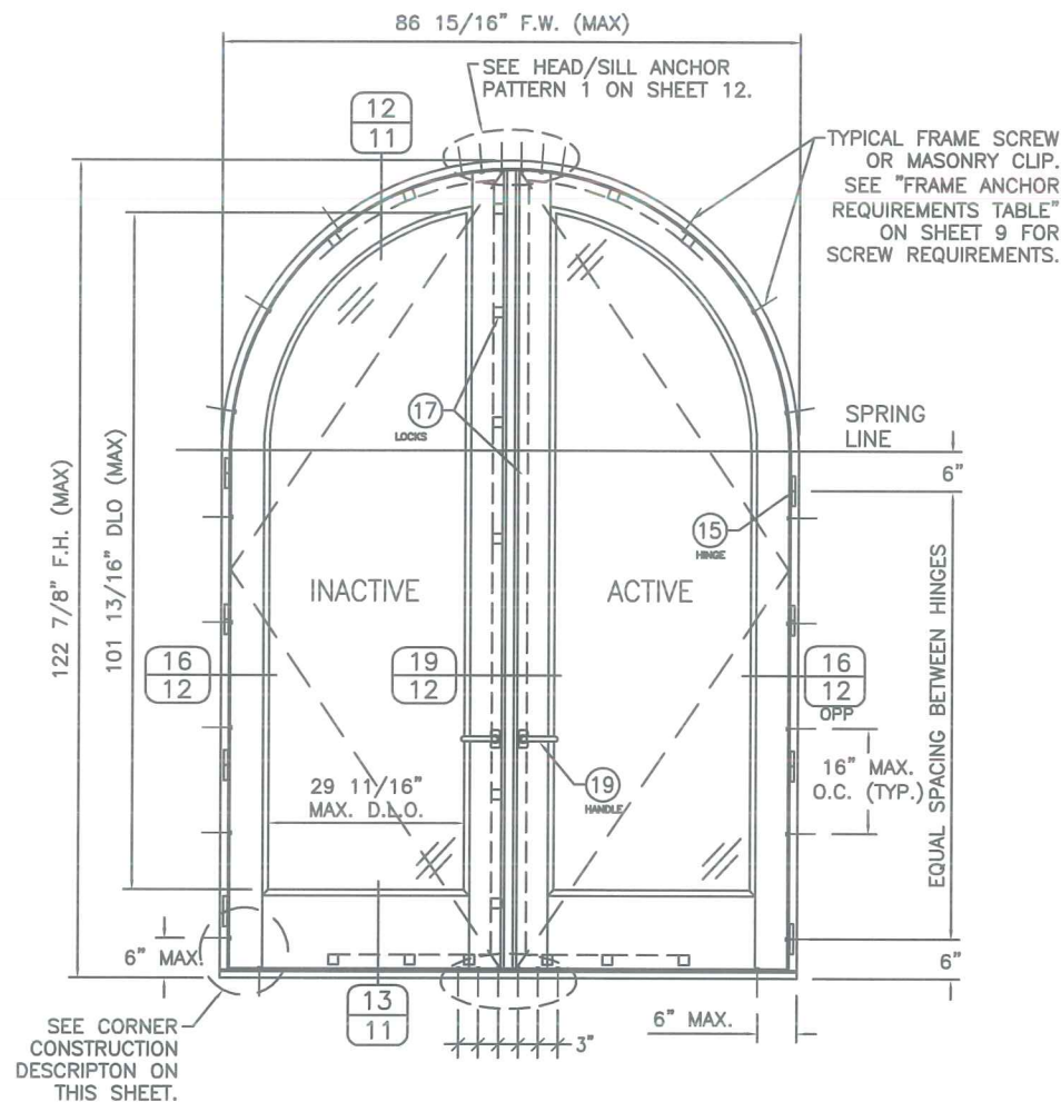
DOUBLE HALF ROUND DOOR (EXTERIOR VIEW)
