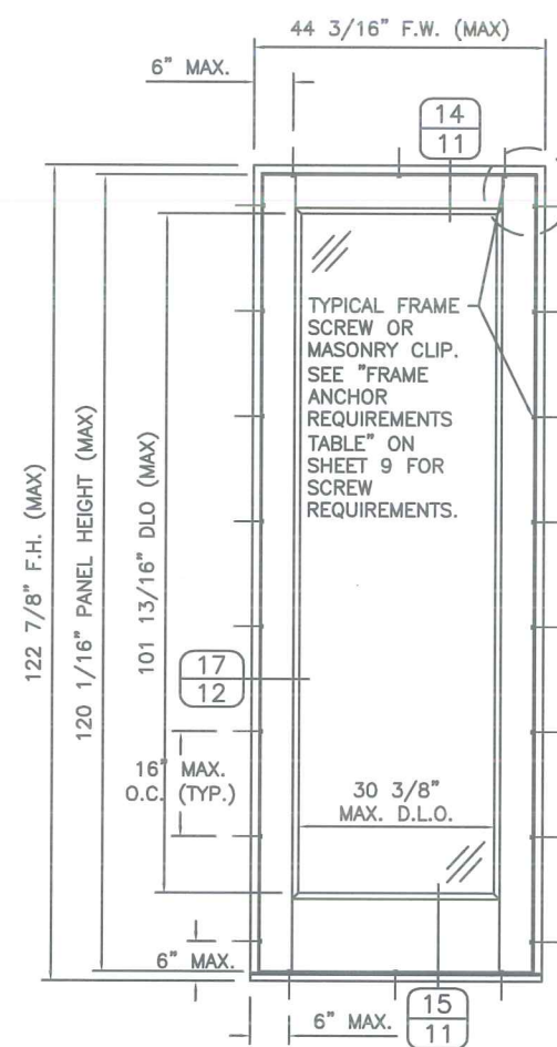
OPTIONAL SINGLE FIXED PANEL (EXTERIOR VIEW)
