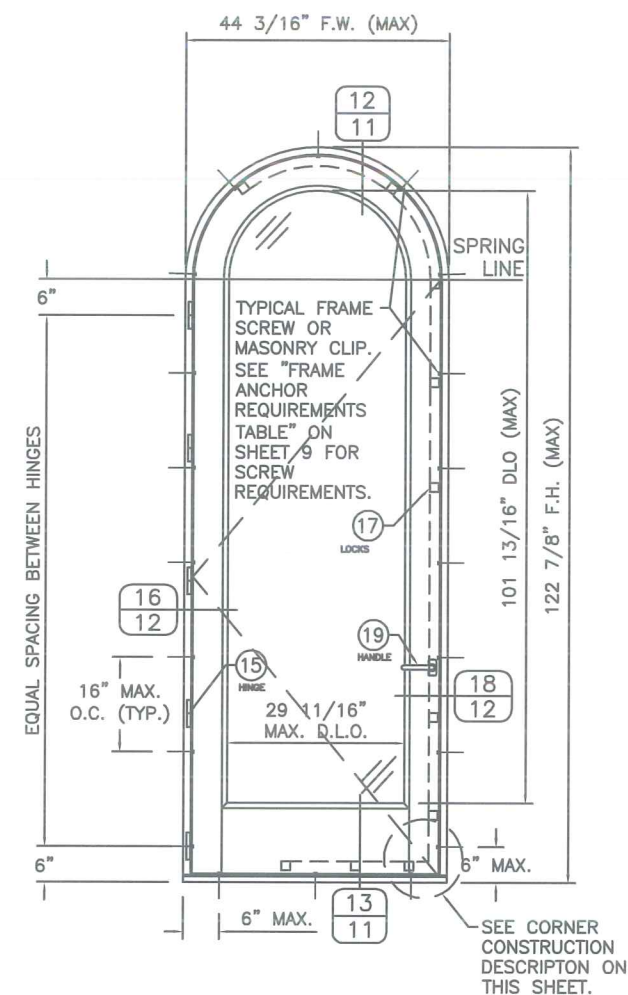
SINGLE HALF ROUND DOOR (EXTERIOR VIEW)
