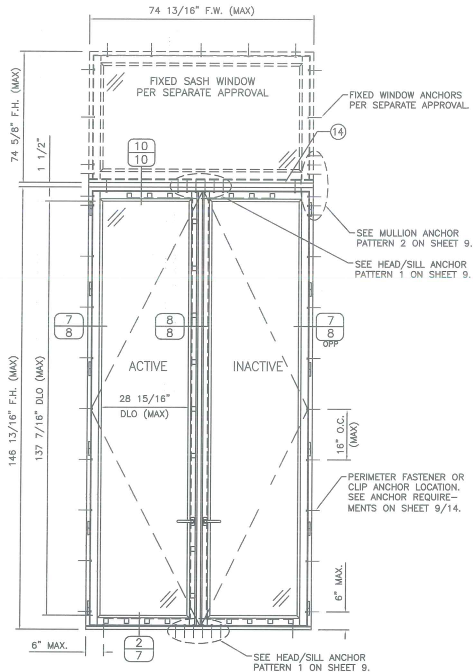
DOUBLE RECTANGULAR DOOR WITH TRANSOM (EXTERIOR VIEW)
