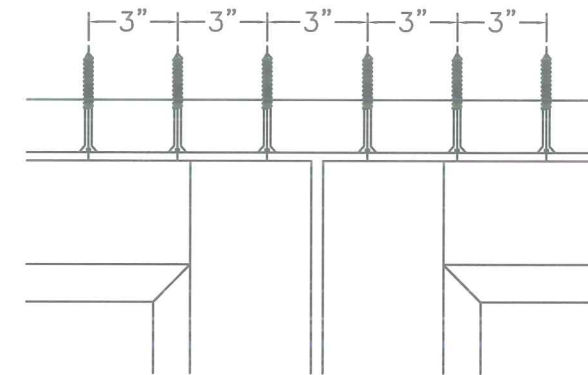
HEAD ANCHOR PATTERN 1 (SILL SIMILAR)
