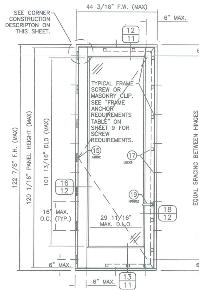
SINGLE RECTANGULAR DOOR (EXTERIOR VIEW)
