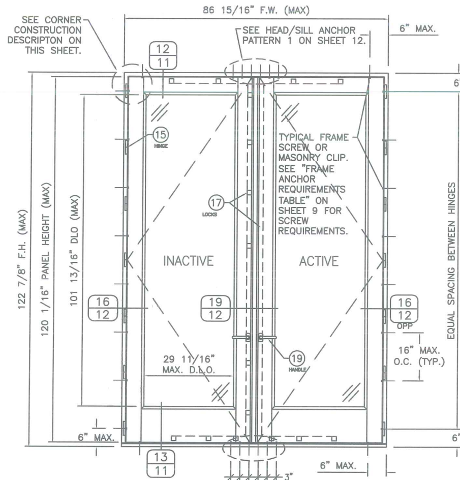
DOUBLE RECTANGULAR DOOR (EXTERIOR VIEW)
