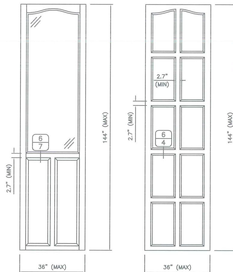
PARTIAL RAISED PANELS WITH STANDARD MID-RAILS (EXTERIOR VIEW)
