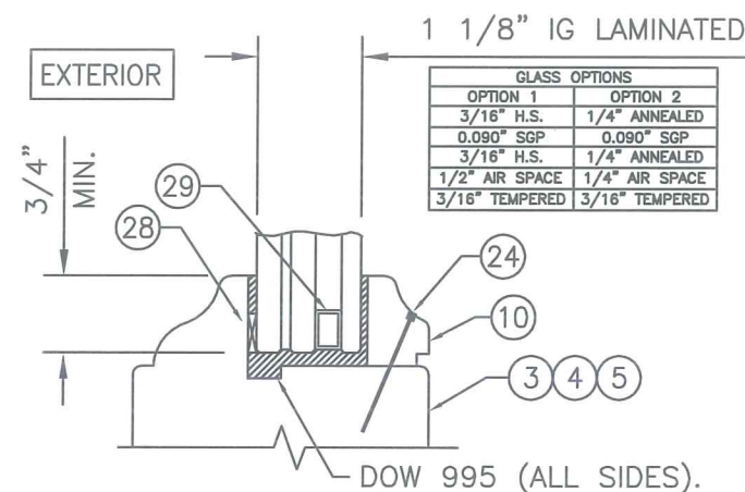
1 1/8" INSULATED LAMINATED GLASS TYPE B
