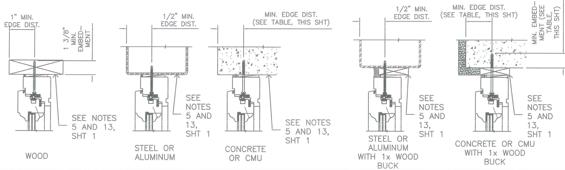
TYPICAL ANCHOR CONDITIONS
