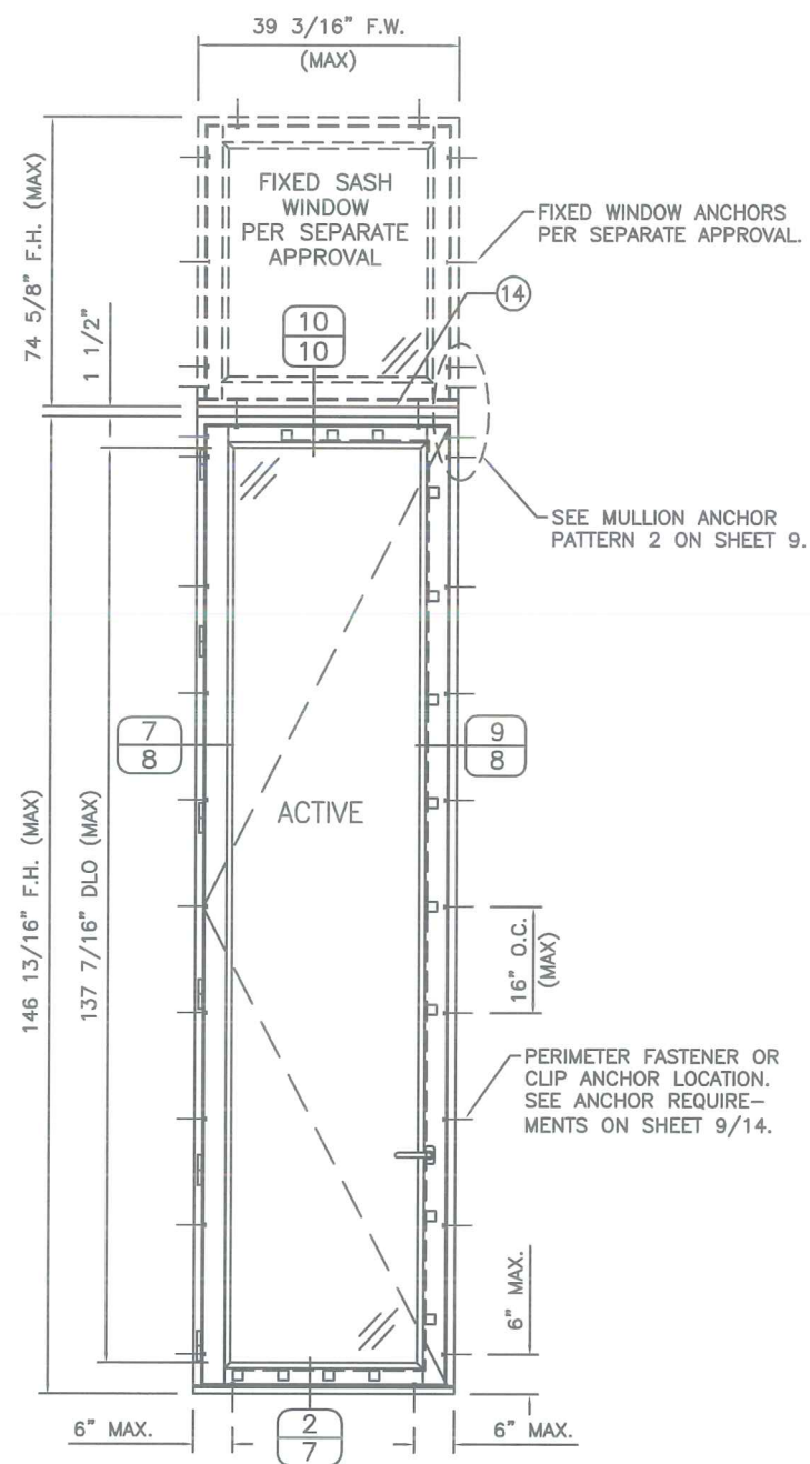
SINGLE RECTANGULAR DOOR WITH TRANSOM (EXTERIOR VIEW)
