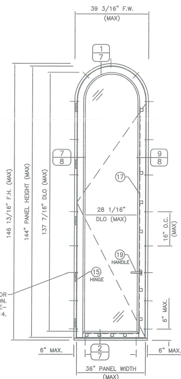
SINGLE HALF ROUND DOOR (EXTERIOR VIEW)
