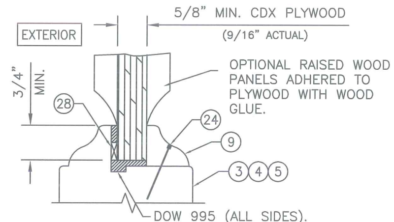
PARTIAL WOOD PANEL TYPE C
