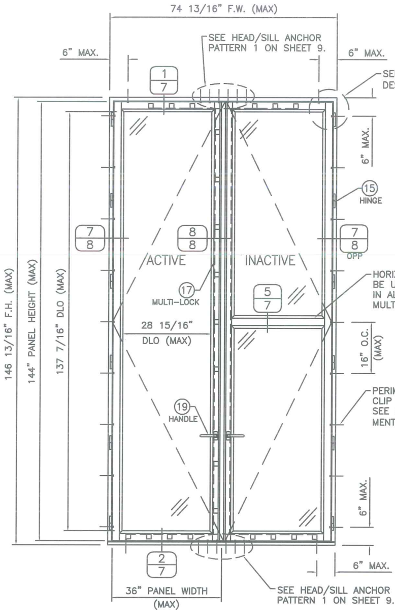
DOUBLE RECTANGULAR DOOR (EXTERIOR VIEW)
