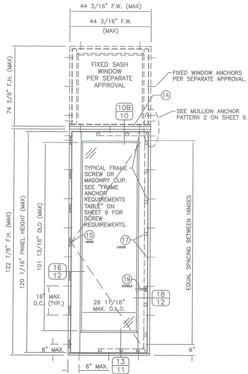
SINGLE RECTANGULAR DOOR WITH TRANSOM (EXTERIOR VIEW)
