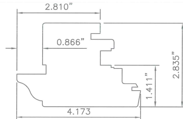
④ ACTIVE MEETING STILE
