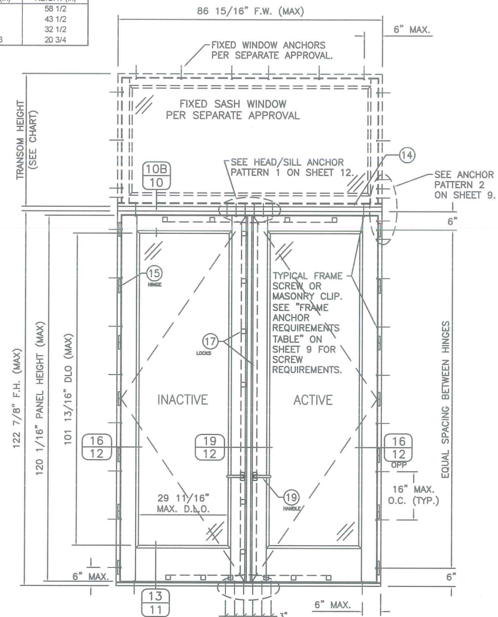
DOUBLE RECTANGULAR DOOR WITH TRANSOM (EXTERIOR VIEW)
