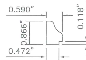
⑩ INSULATED GLASS STOP
