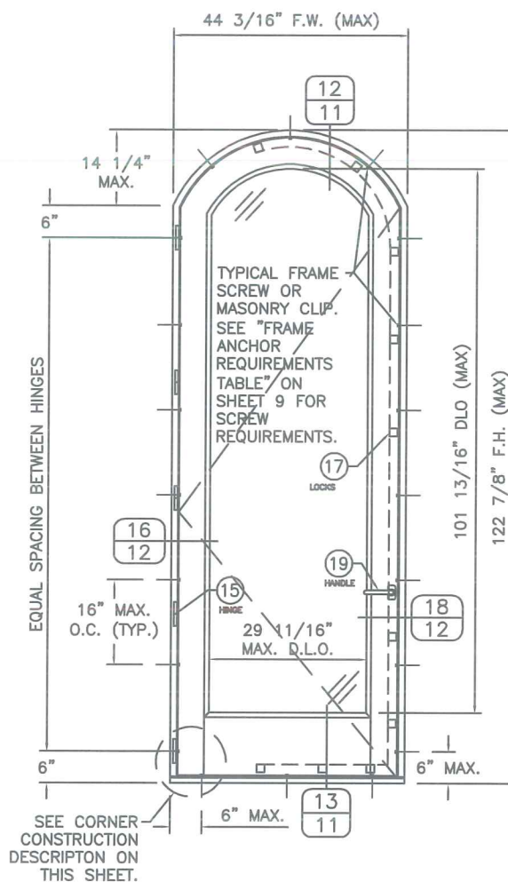
SINGLE ARCH TOP DOOR (EXTERIOR VIEW)
