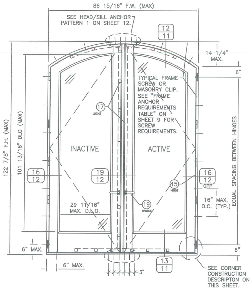
DOUBLE ARCH TOP DOOR (EXTERIOR VIEW)
