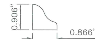
⑨ GLASS/PANEL STOP
