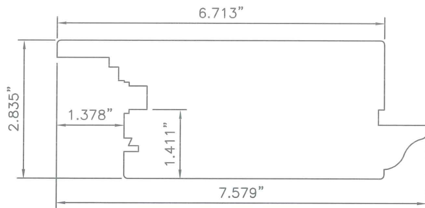
30 INACTIVE MEETING STILE
